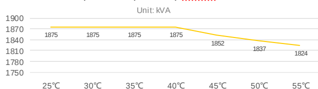
Temperature (Celsius) Derate Curves
