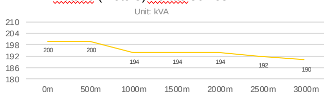
Altitude (meters) Derate Curves
