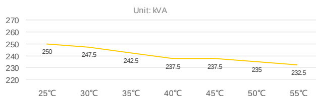
Temperature (Celsius) Derate Curves
